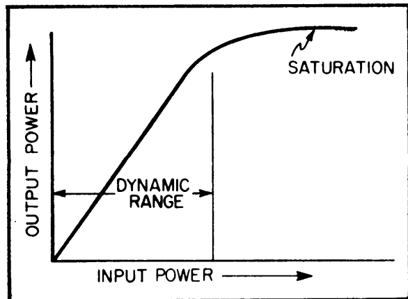
Figure 4-37. Linear Receiver.
