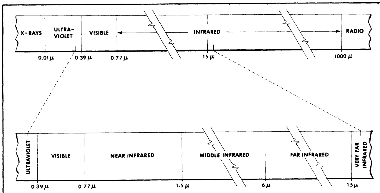
Figure 4-42. The Optical Spectrum.
