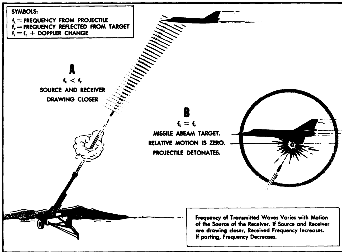
Figure 6-7. Radar Proximity Fused Projectile.
