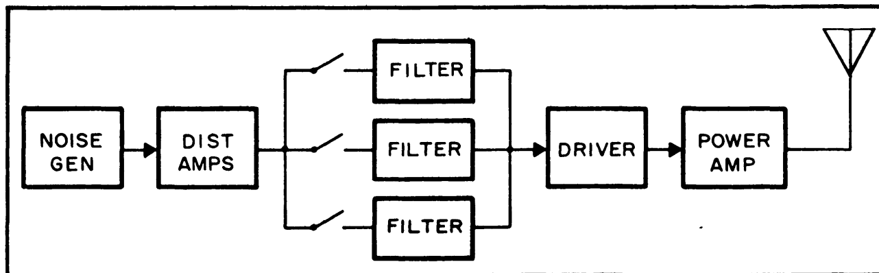
Figure 4-20. Barrage Transmitter.
