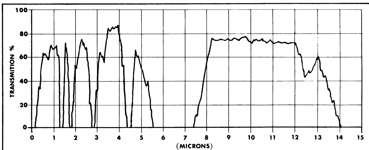
Figure 4-43. Atmospheric Transmission.
