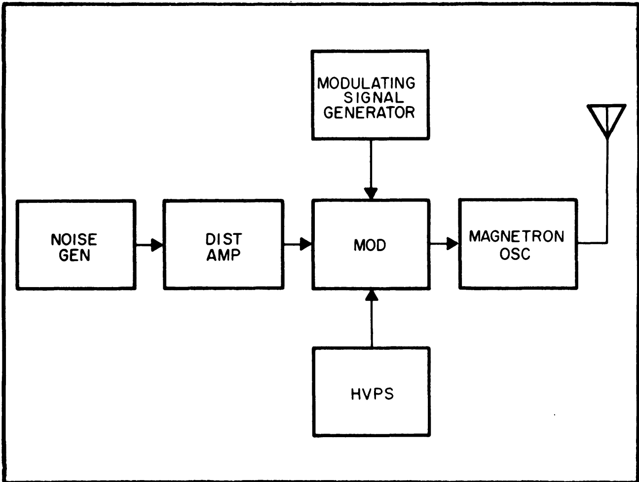
Figure 4-23. Basic Modulated Transmitter.
