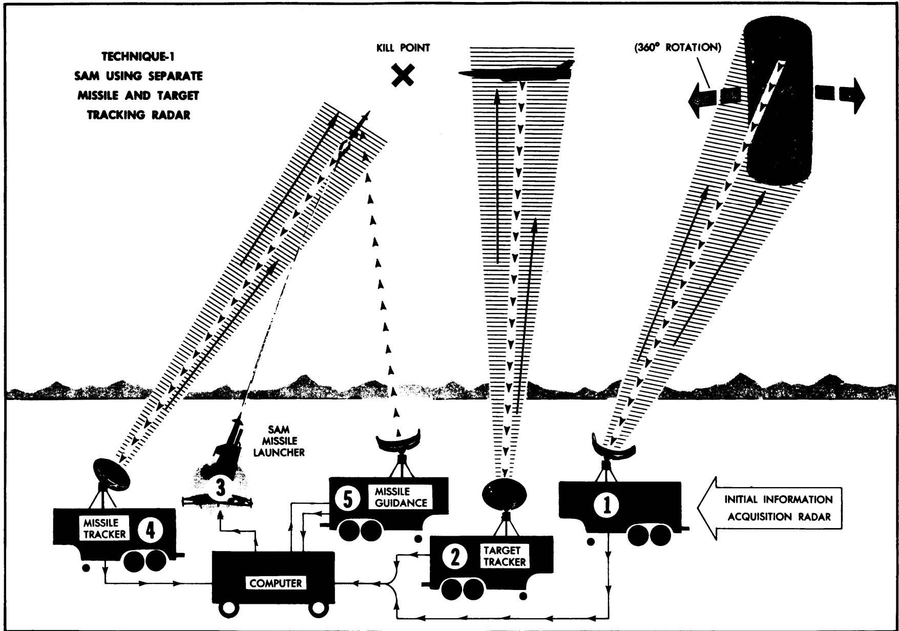
Figure 6-3. SAM Using Missile and Target Tracking.
