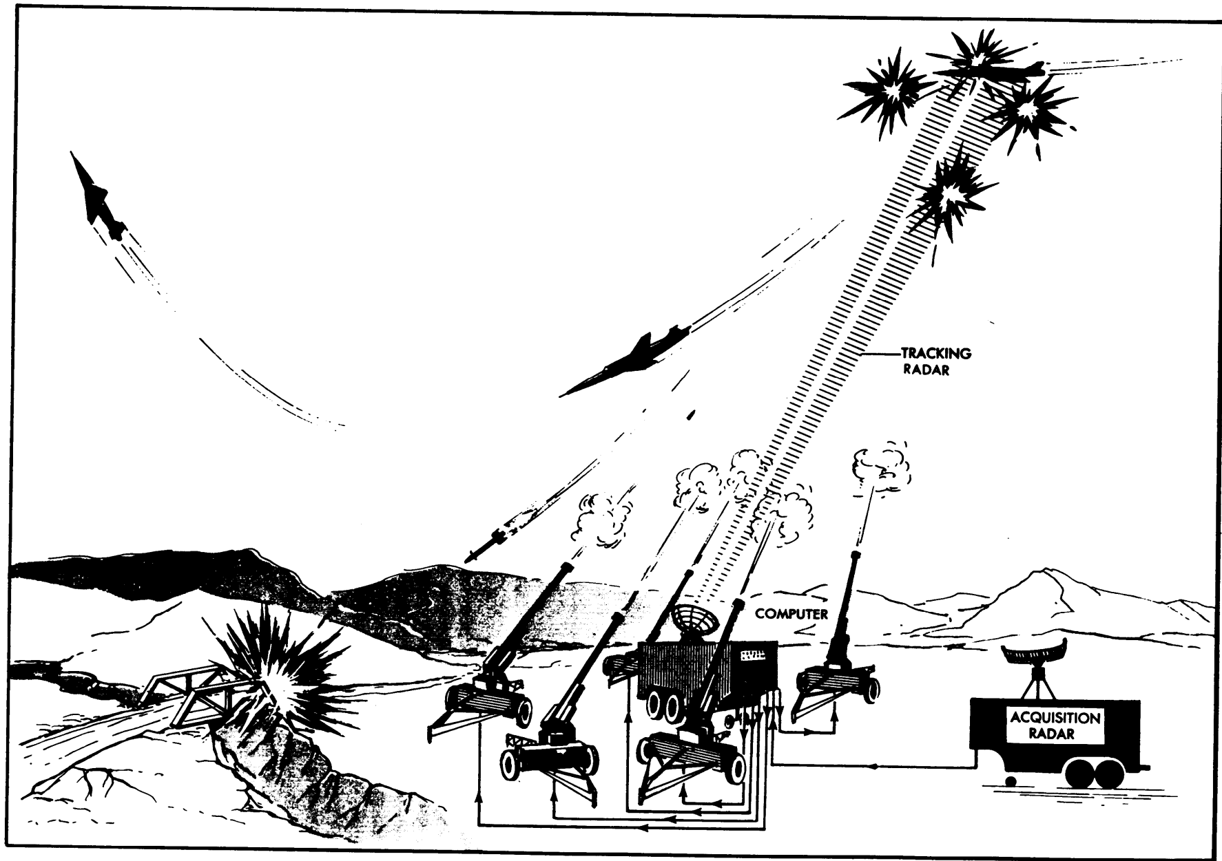
Figure 6-6. Typical AAA Battery Layout.
