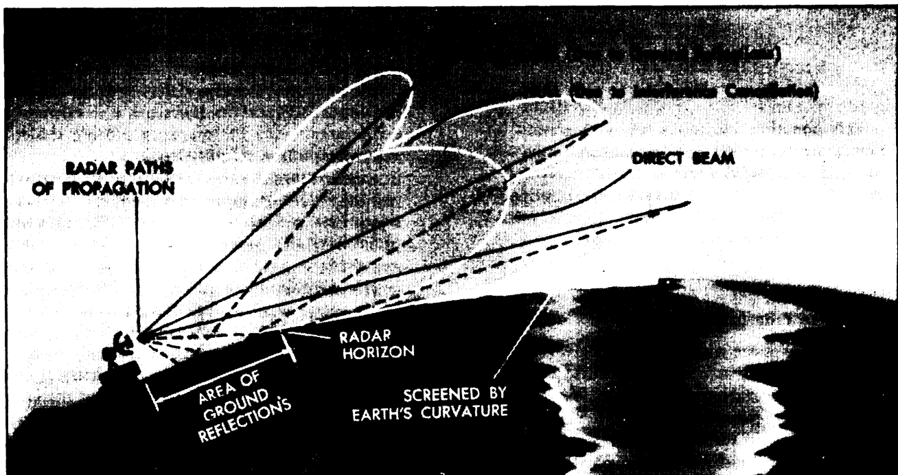
Figure 2-15. Nonstandard Propagation.
