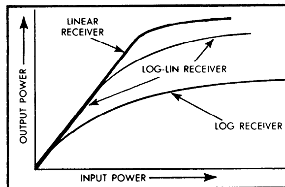
Figure 4-38. Comparison of Receiver Responses.
