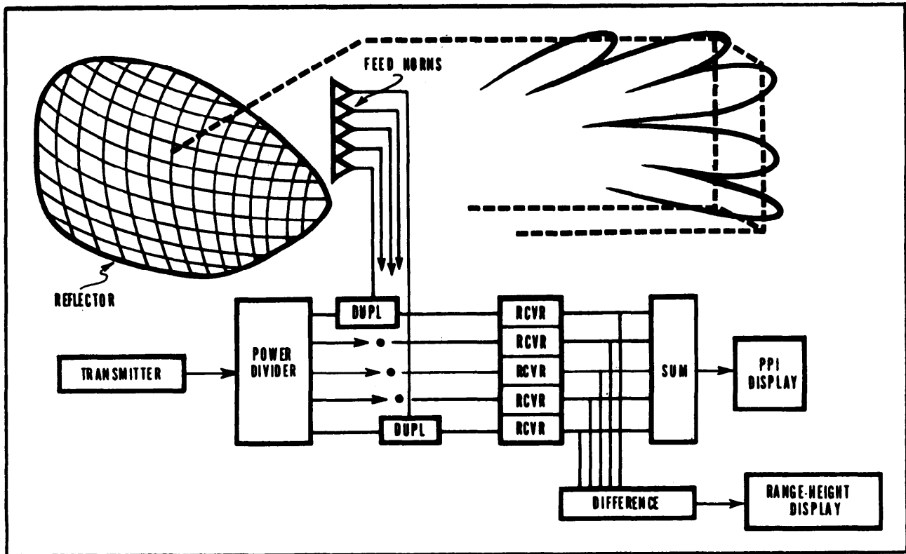
Figure 2-21. Stacked Beam Radar.
