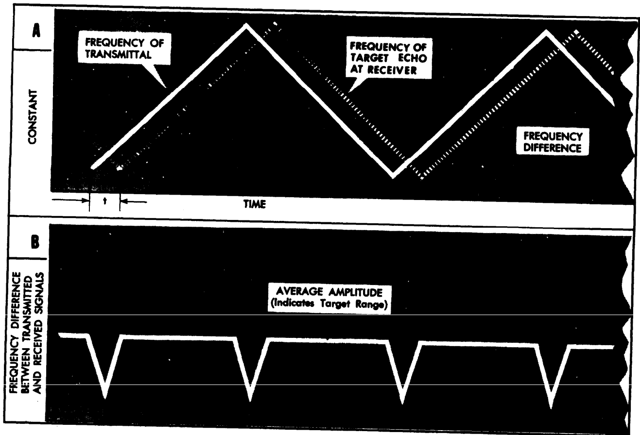
Figure 2-31. Stationary Target.
