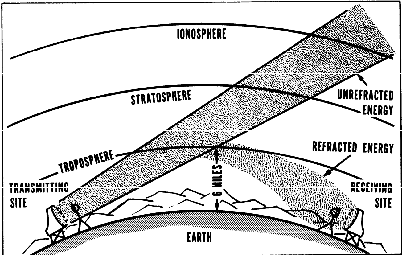
Figure 2-7. Forward Tropospheric Scattering Principle.
