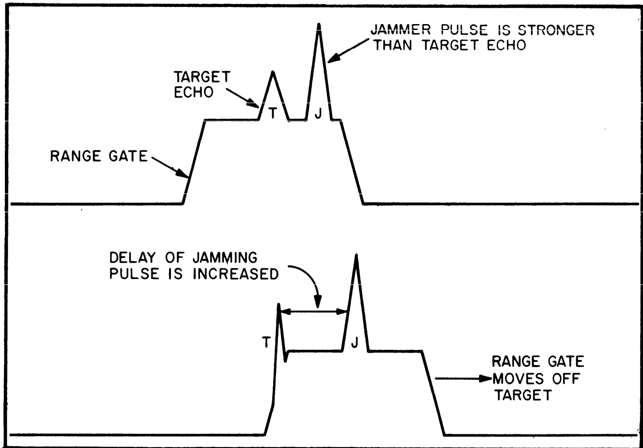
Figure 4-25. Range Gate Stealer.
