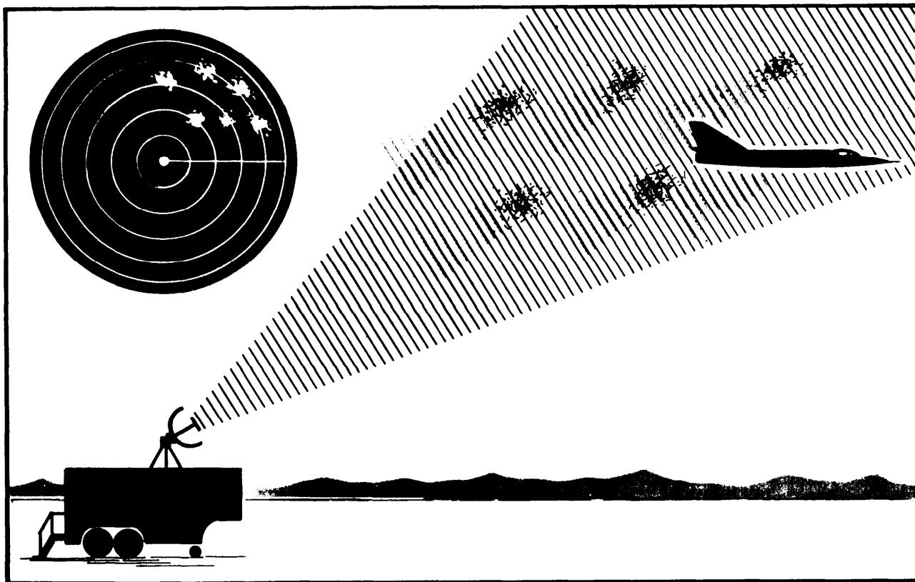
Figure 4-28. Random Chaff Dispensing.
