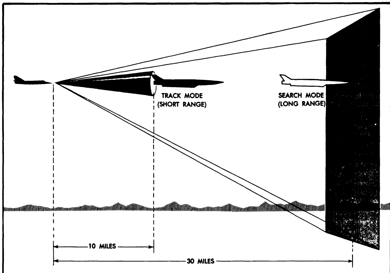
Figure 6-1. AI Search Mode vs Track Mode.
