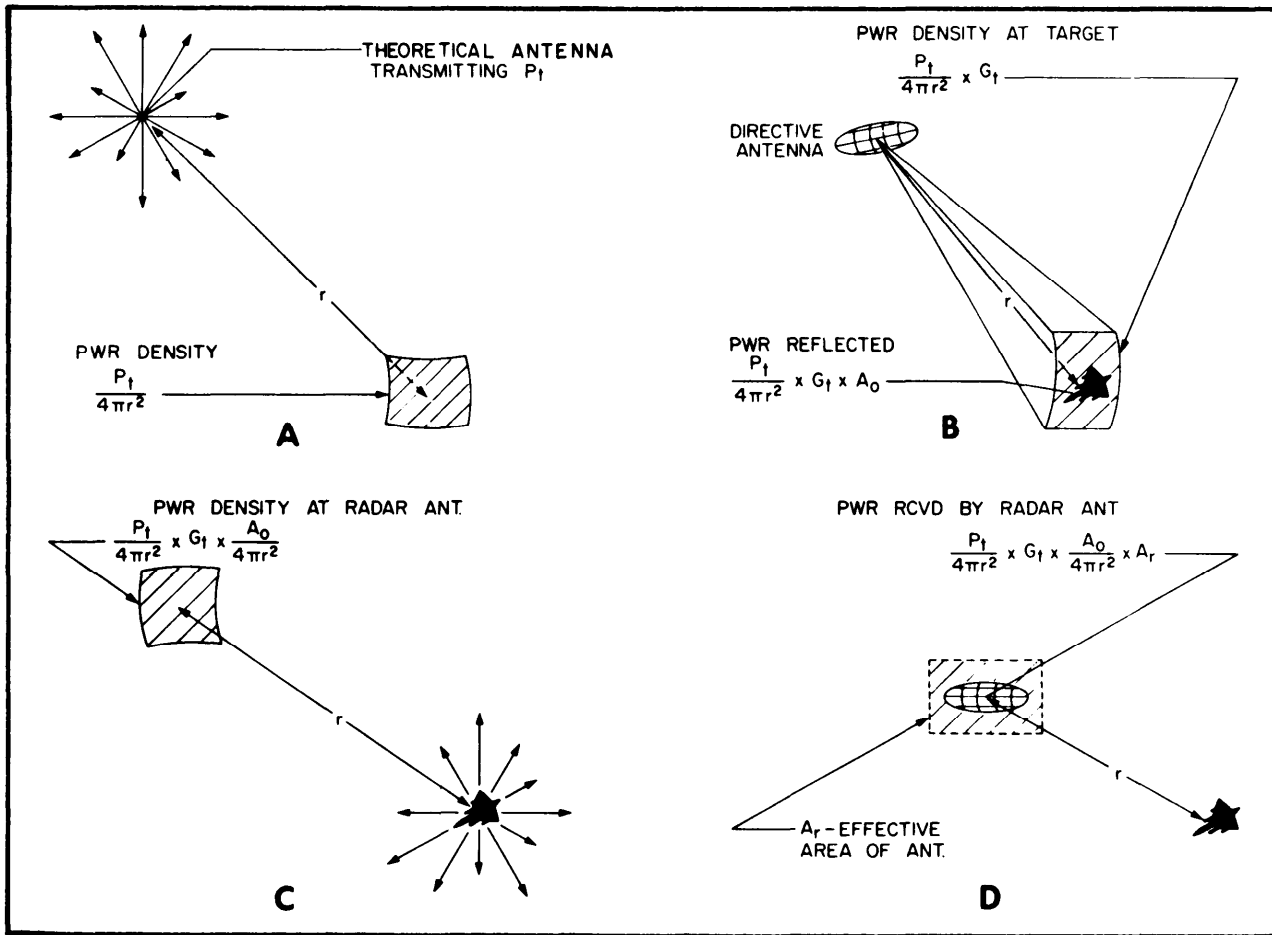
Figure 2-14. Free Space Radar Equation.
