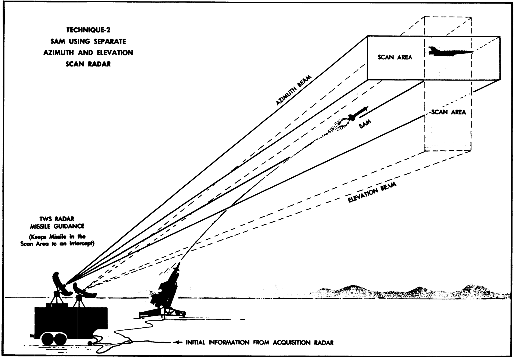
Figure 6-4. SAM Using Track-While-Scan.
