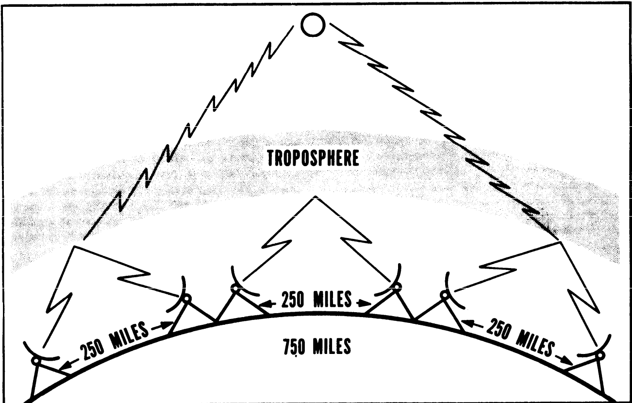
Figure 2-8. Troposcatter vs Satellite Communication.
