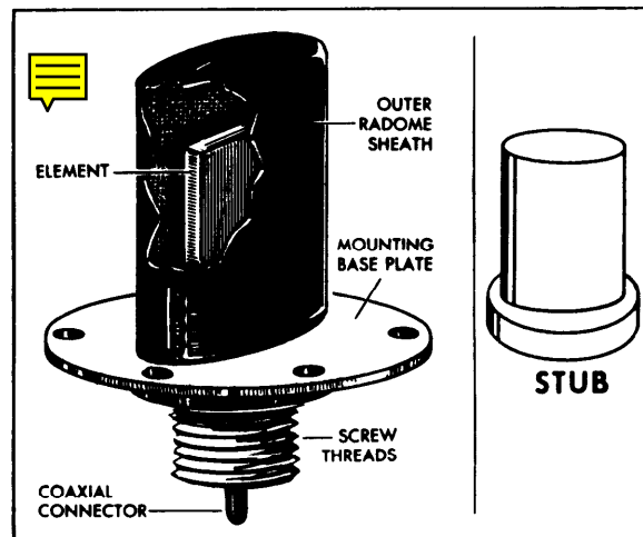
Figure 4-6. Stub/Blade Antenna.
