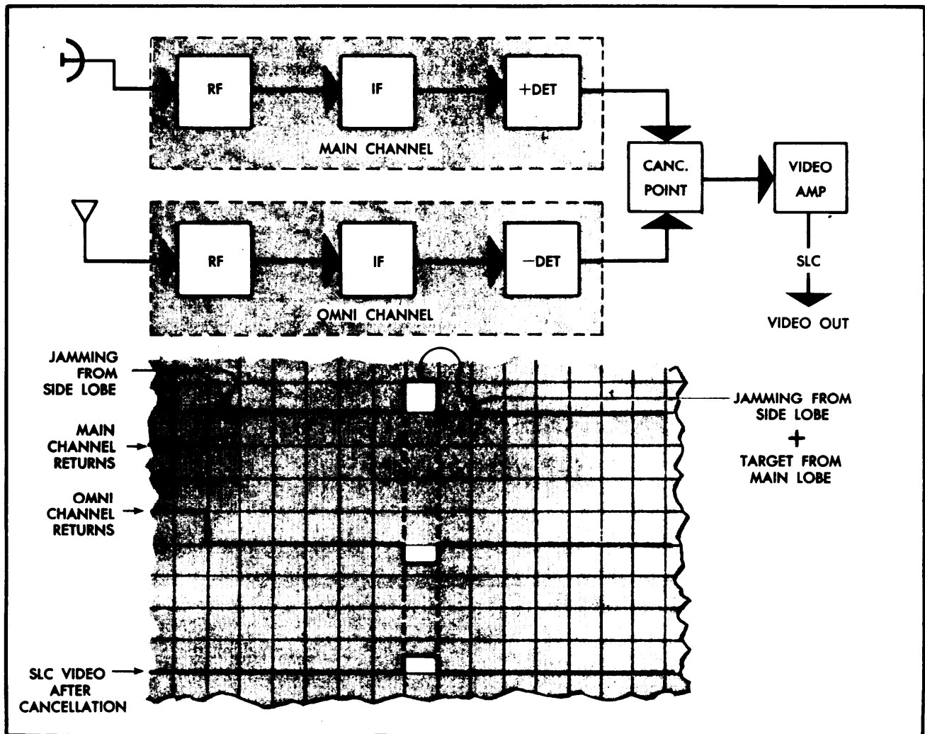
Figure 4-41. SLC Block Diagram and Waveforms.
