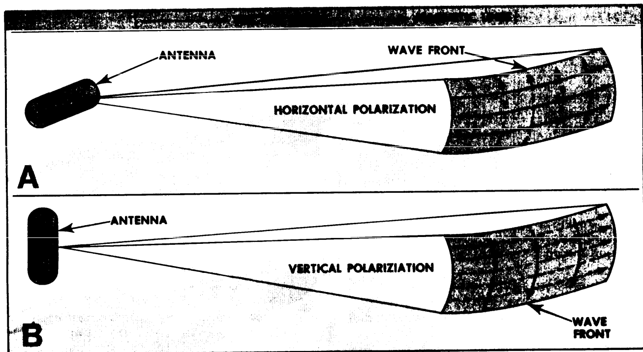
Figure 4-8. Vertical and Horizontal Polarization.
