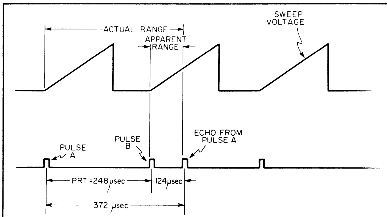
Figure 2-11. Second-Time-Around Echo.
