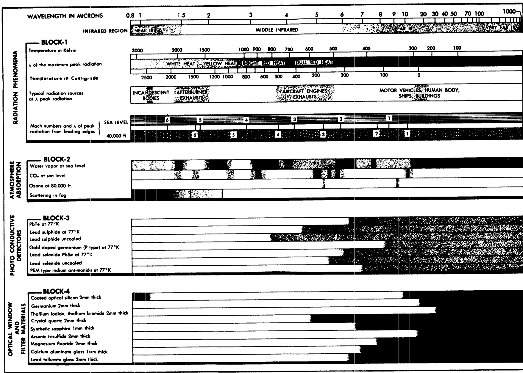
Figure 4-44. IR Data Chart.
