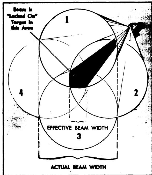
Figure 2-22. Conical Scan.
