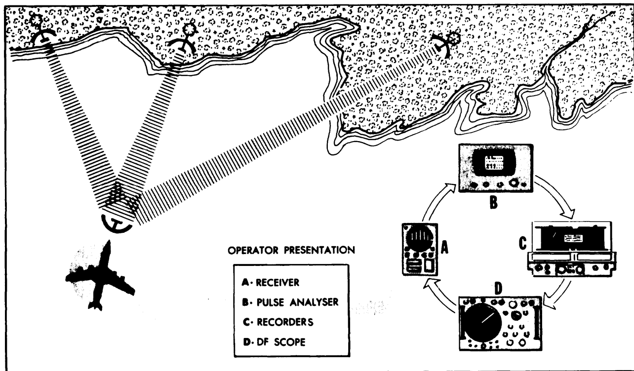
Figure 4-1. ESM Sensor.
