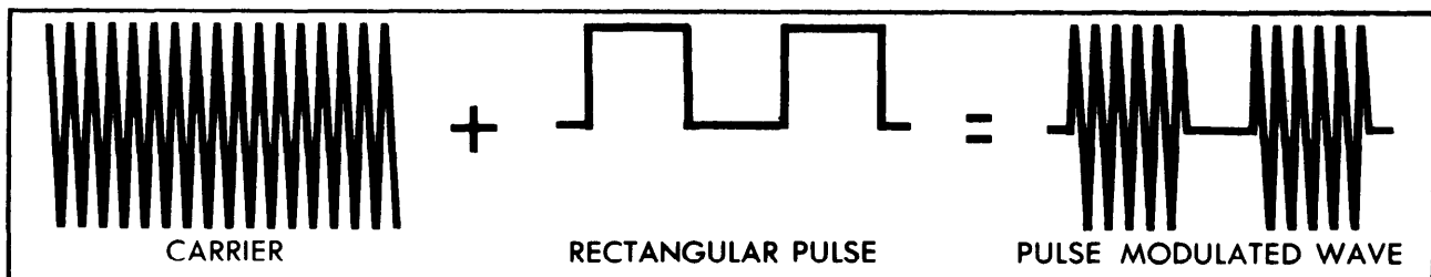
Figure 2-6. Pulse Modulation.
