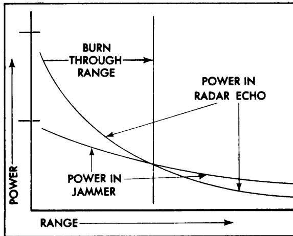
Figure 4-14. Burn-Through Range.
