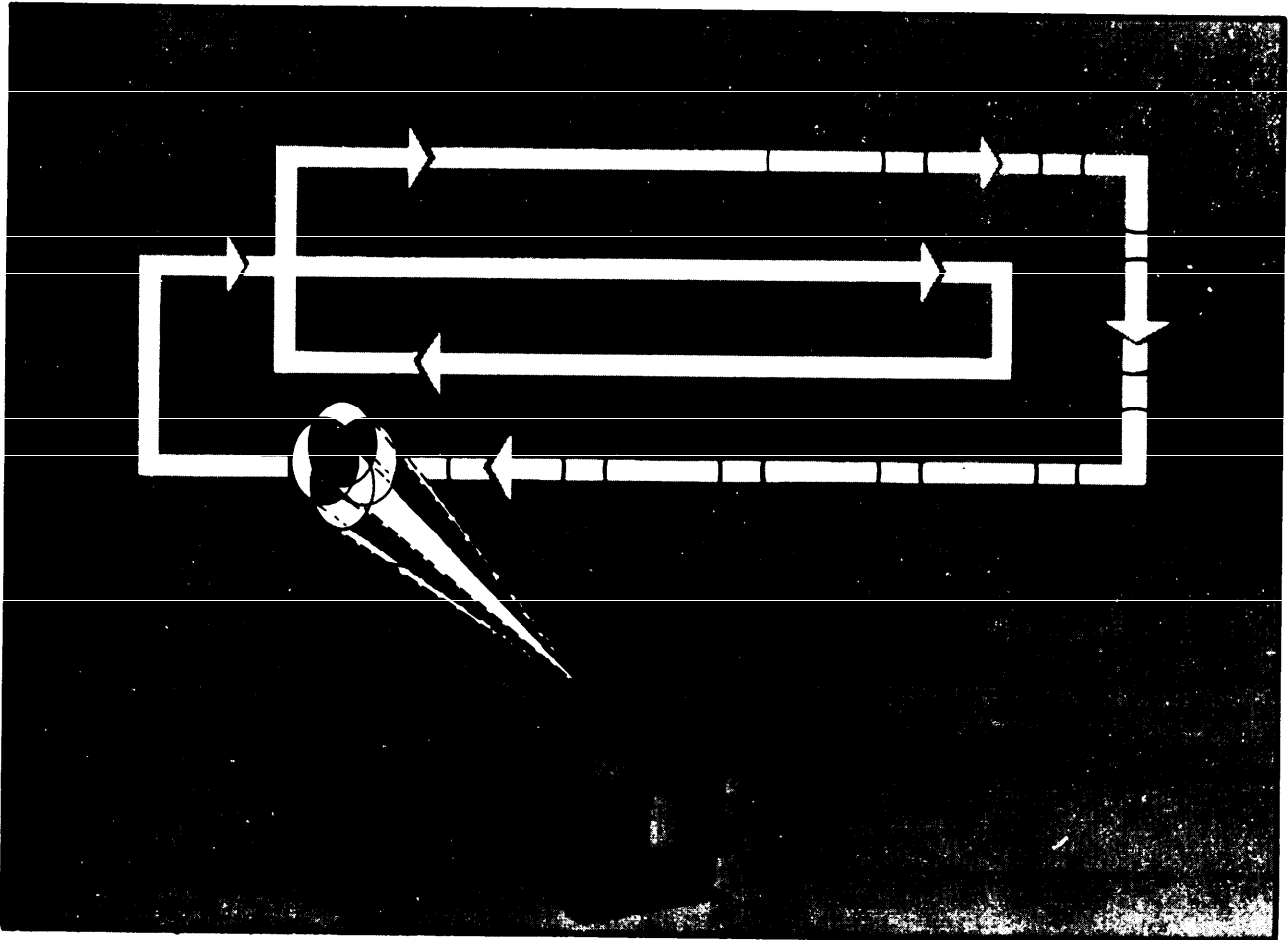
Figure 2-27. Palmer-Raster Scan.
