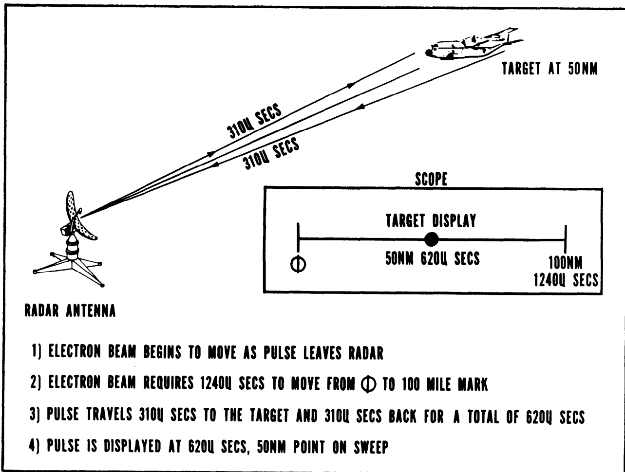
Figure 2-9. Determining Range.
