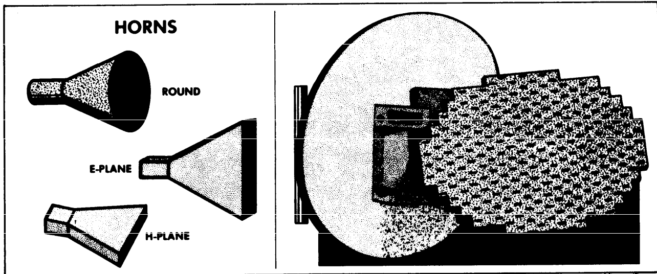
Figure 4-7. Horn and Phased Array Antennas.
