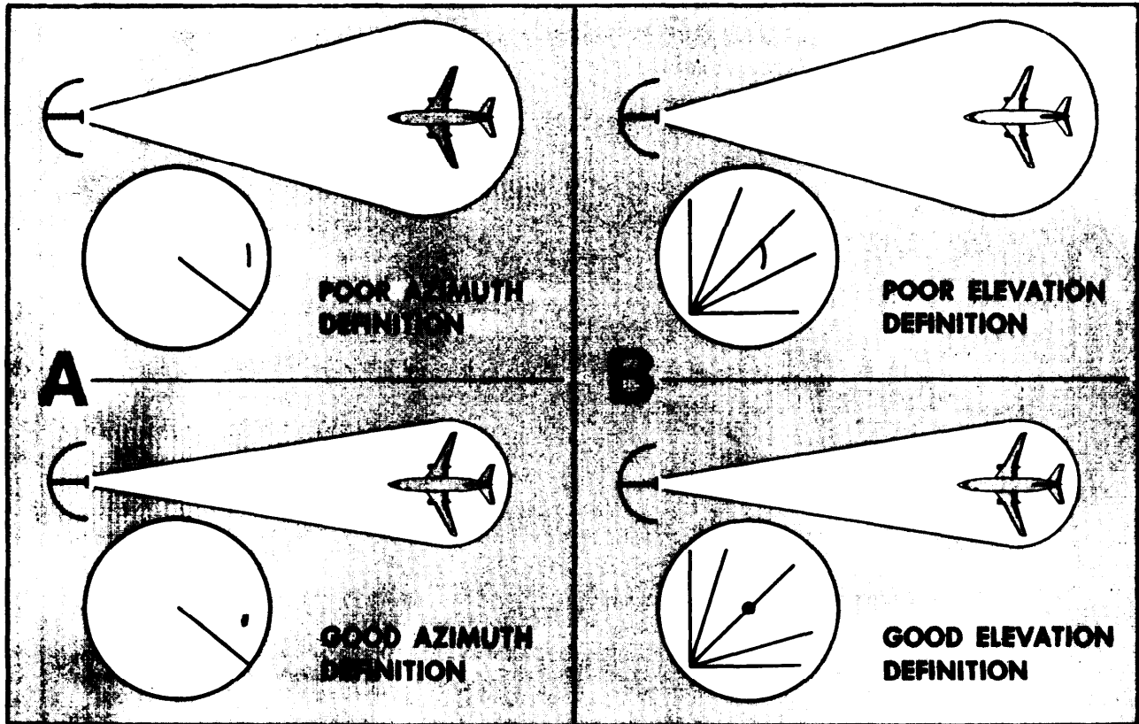
Figure 2-13. Azimuth/Elevation Definition.
