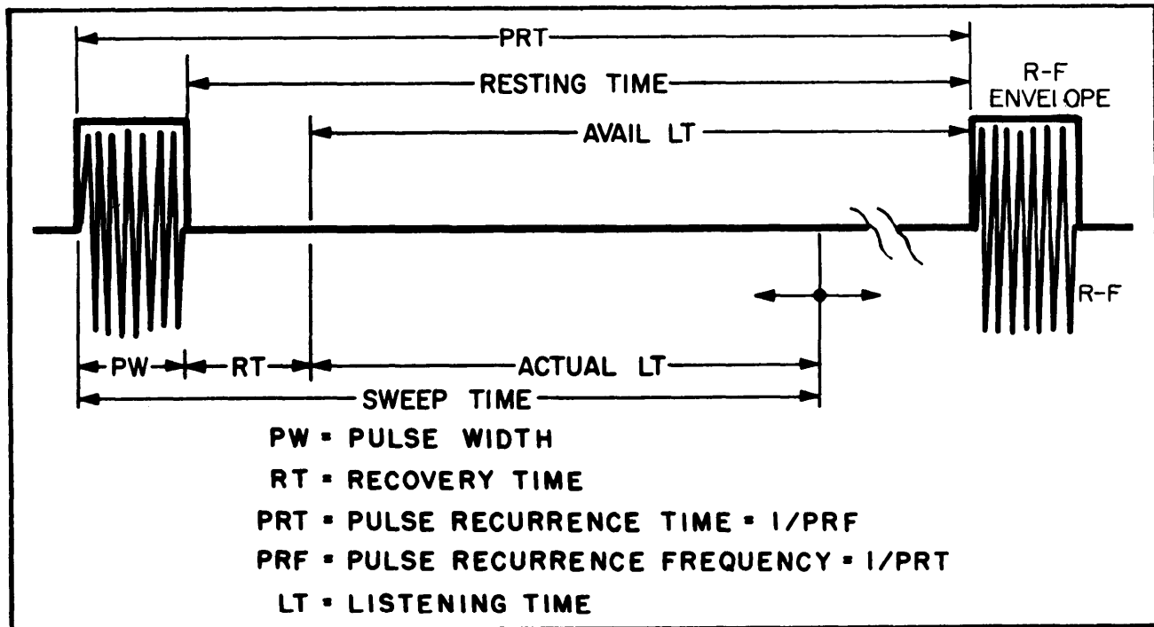
Figure 2-10. Transmissions and Reception Cycle.
