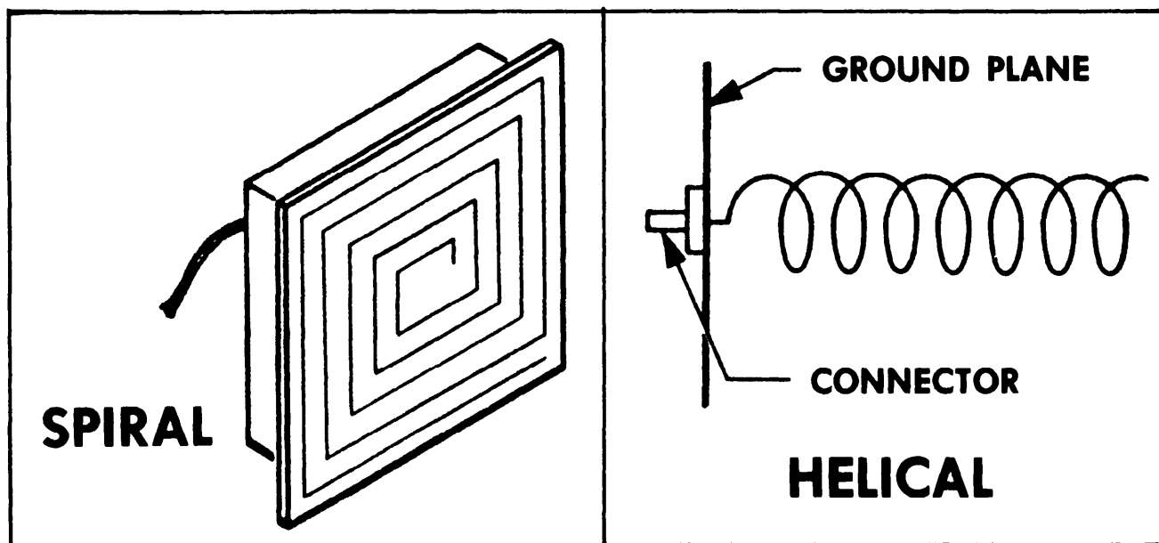
Figure 4-13. Spiral Antenna and Helical Antenna.
