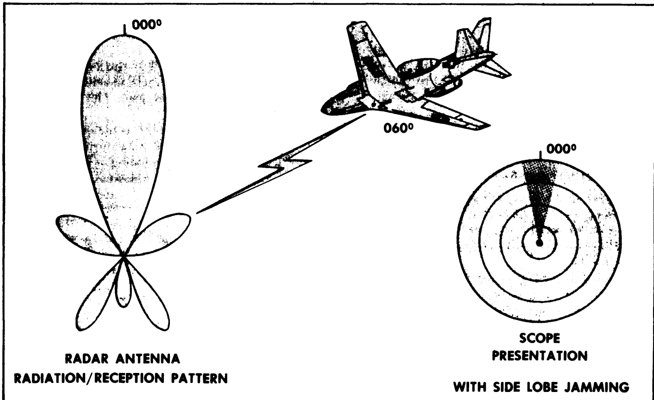
Figure 4-39. Side Lobe Jamming.
