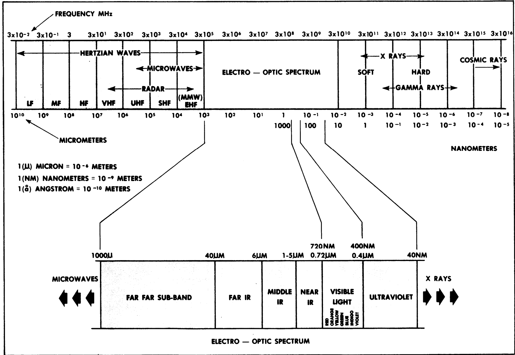
Figure 2-1. Electromagnetic Wave Spectrum.
