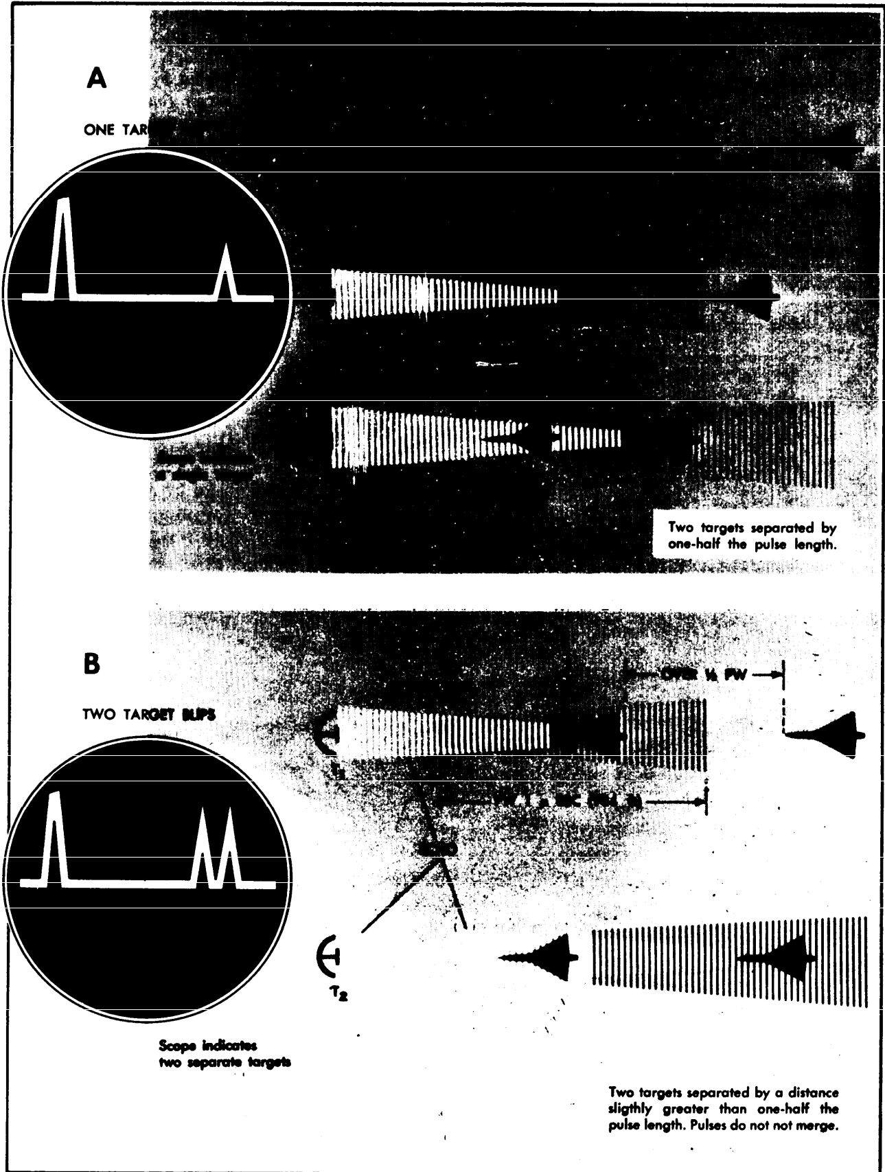
Figure 2-12. Pulse Radar Range Resolution.
