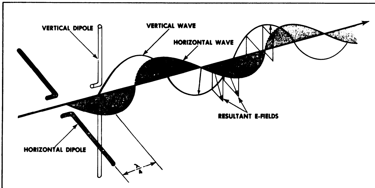
Figure 4-9. Circular Polarization.
