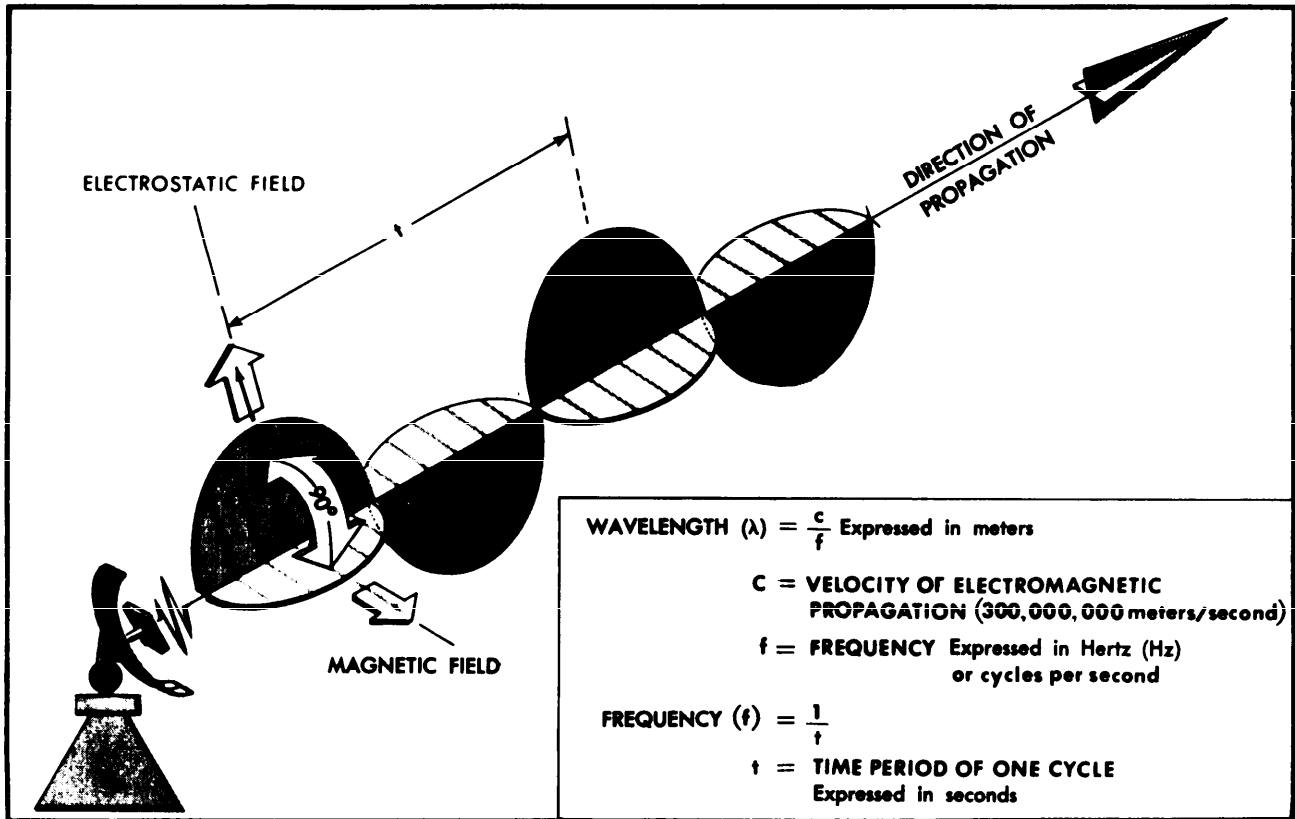
Figure 2-2. Electromagnetic Wave Propagation.
