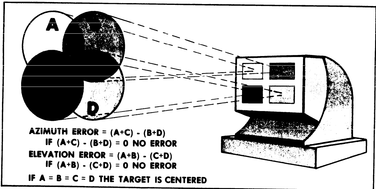
Figure 2-28. Monopulse Radar.
