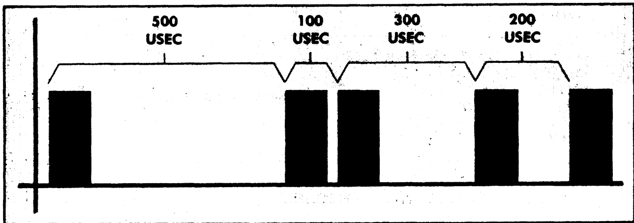
Figure 4-35. Pulsed Radar With Jittered PRF.
