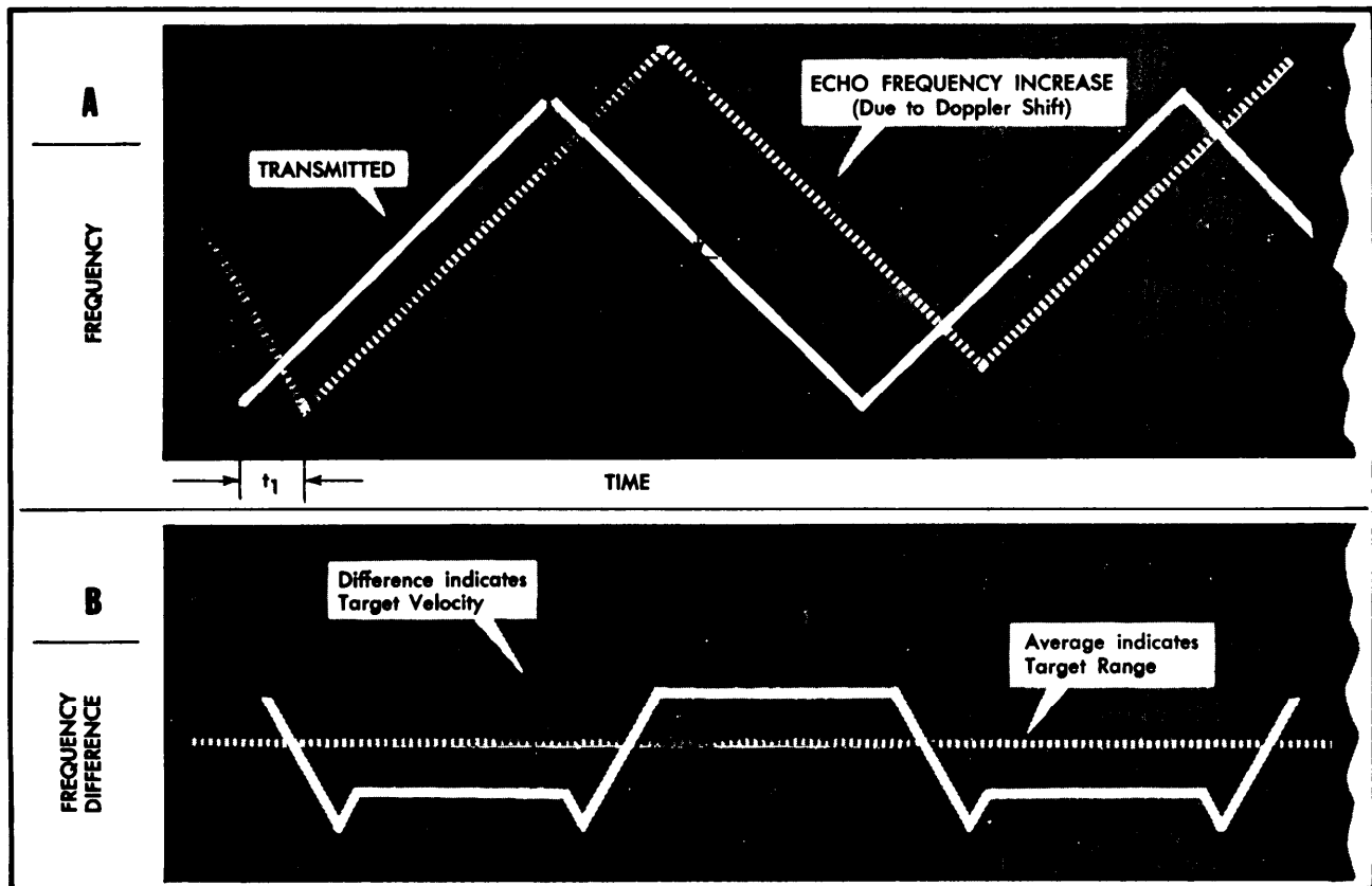
Figure 2-32. Target Moving Toward Radar.
