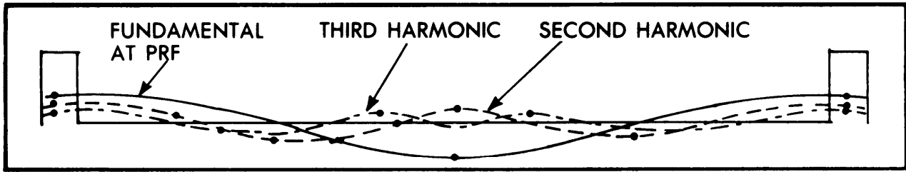
Figure 2-34. Harmonic Content of a Rectangular Waveform.
