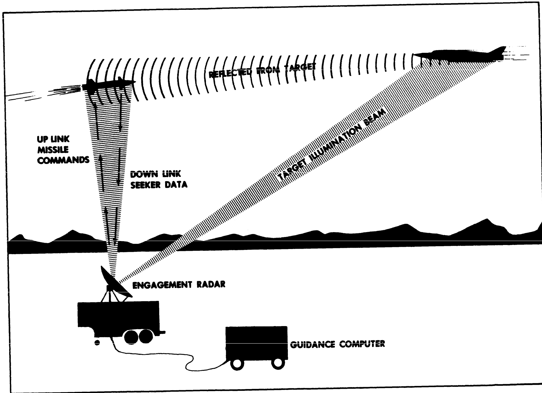
Figure 6-5. Track-Via-Missile Concept.
