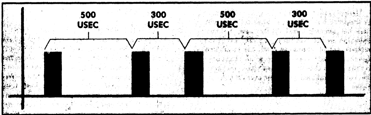
Figure 4-34. Pulsed Radar With Two-Position PRF Stagger.
