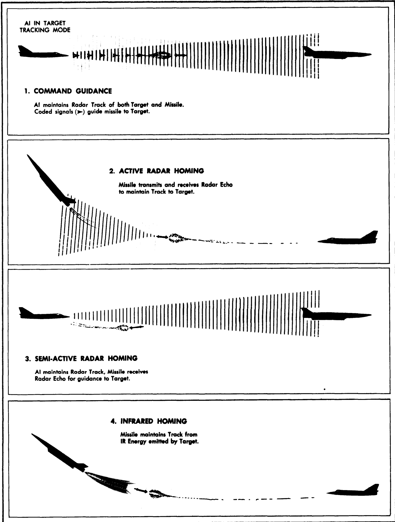
Figure 6-2. Missile Guidance Systems.
