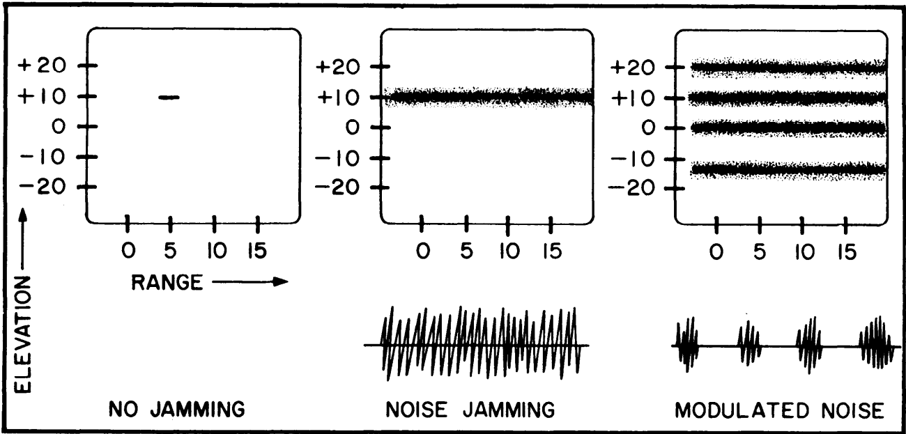
Figure 4-22. Track-While-Scan Jamming.
